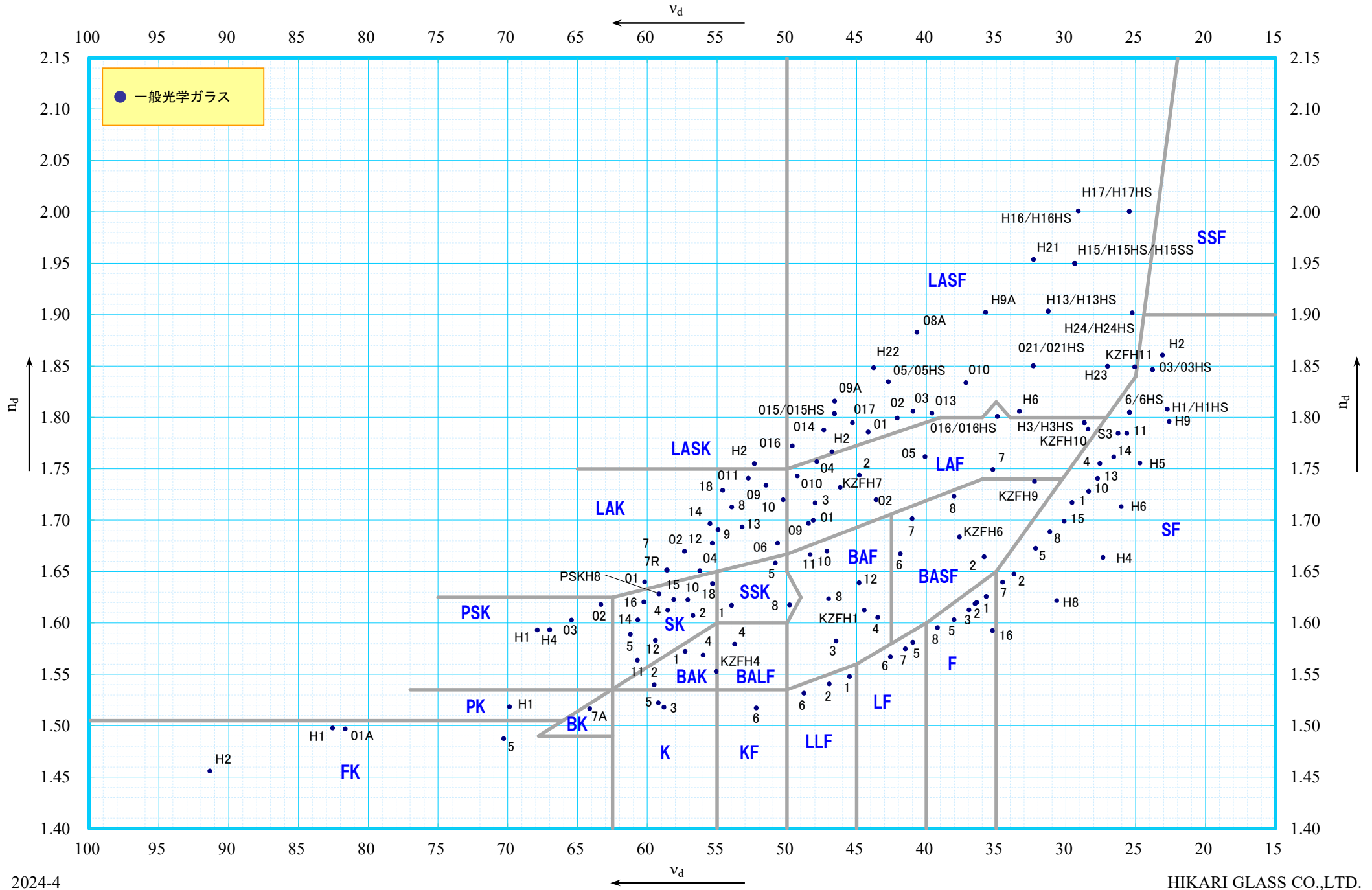
Optical glass n_d - v_d diagram
