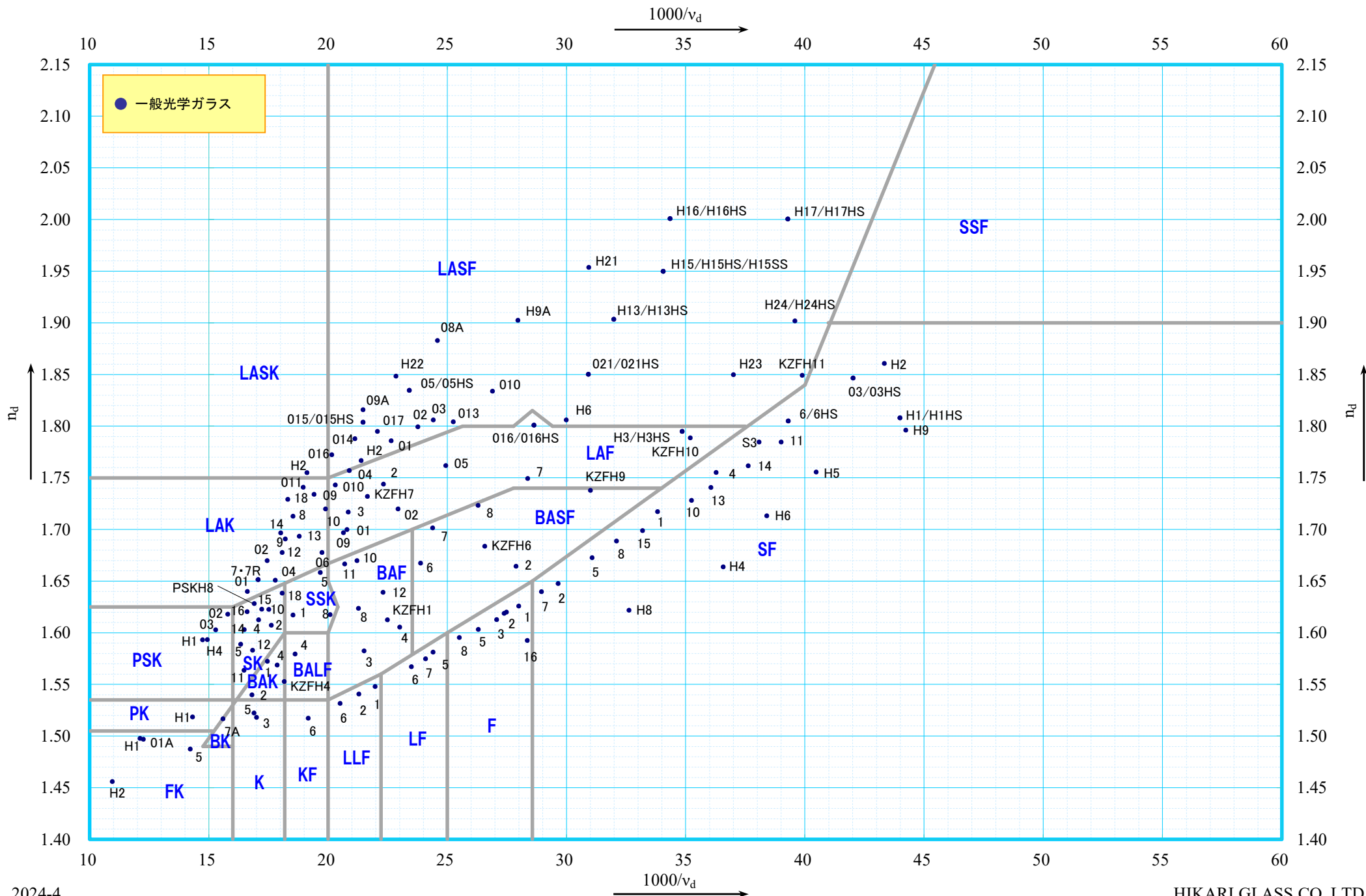
Optical glass n_d-1000/v_d diagram
