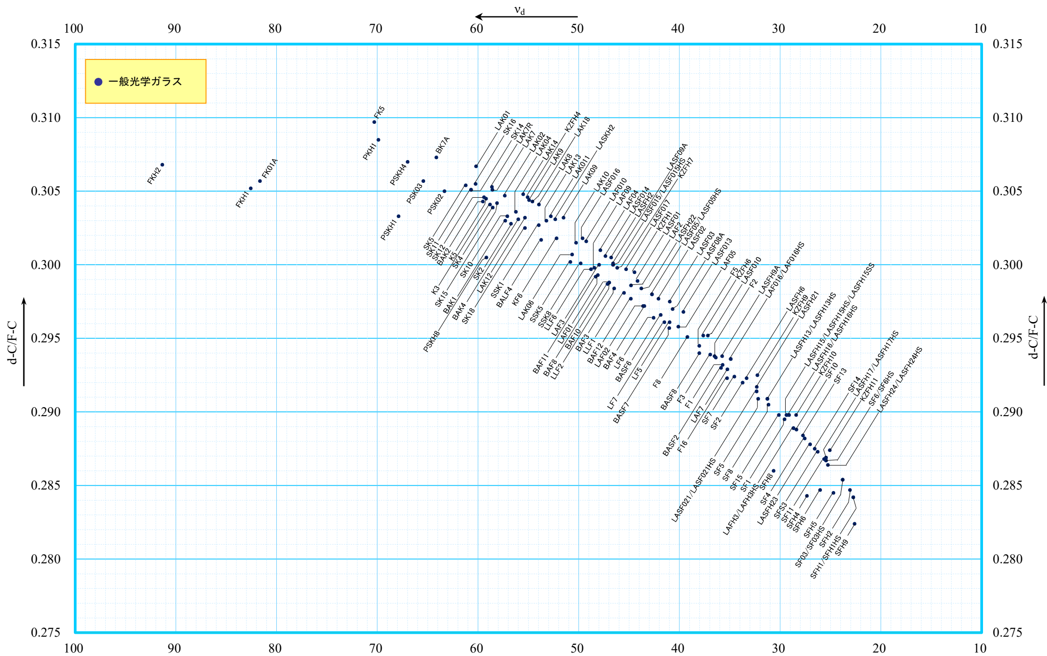
Optical glass d-C/F-C — \nu_d diagram
