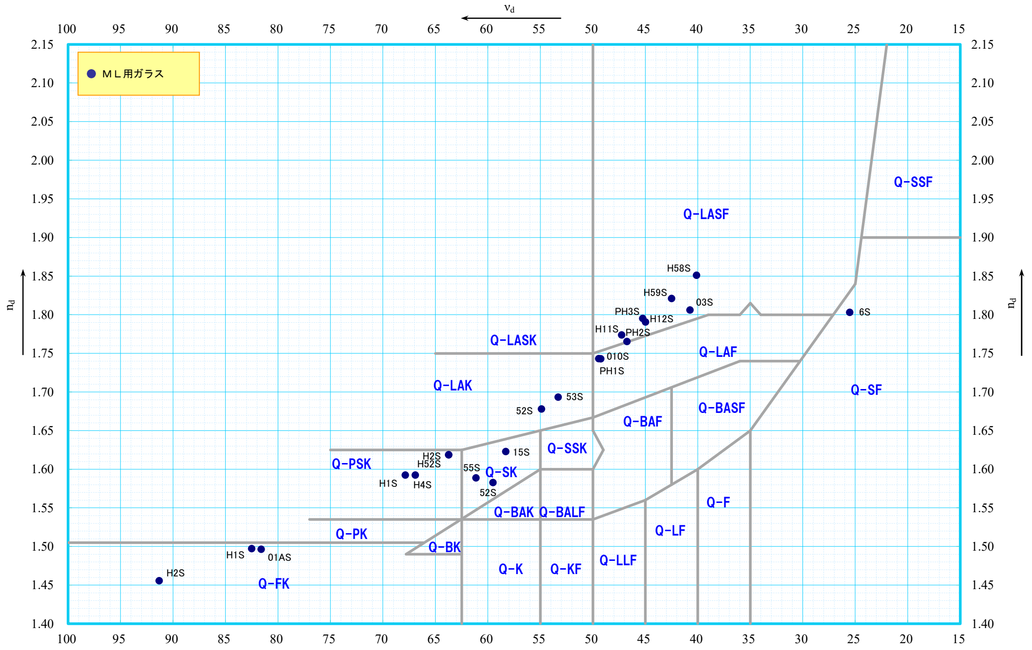
Optical glass for mold lens n_d - v_d diagram
