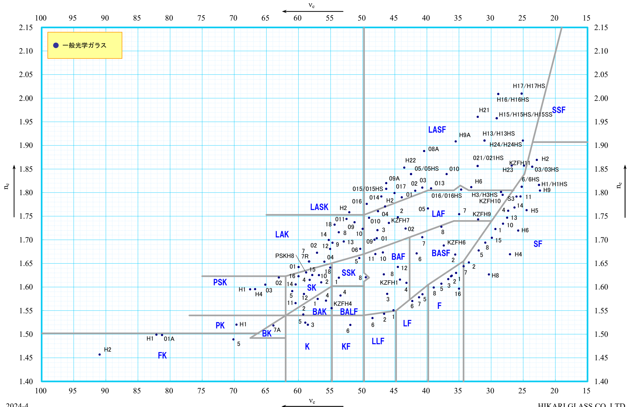
Optical glass n_e - v_e diagram
